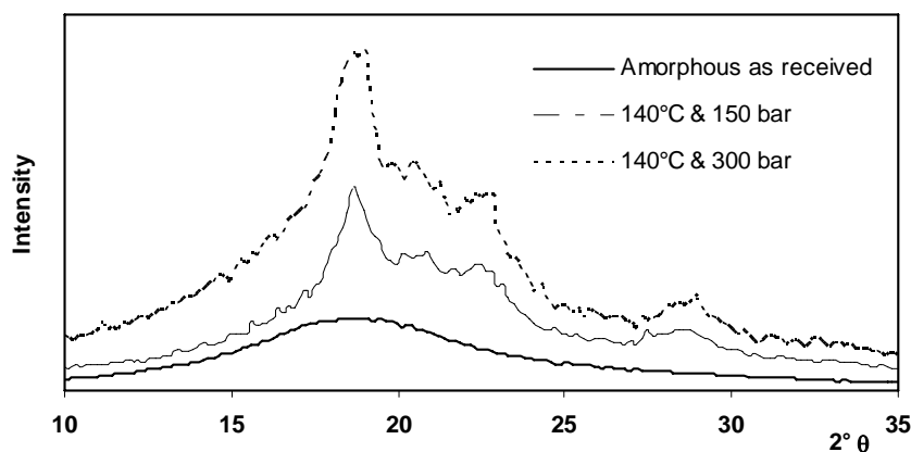
Figure 3. XRD of Amorphous PEEK Films
